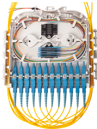
KM 5 (for adapters, up to 12× SC / 24× LC connector, up to 24 splices)
