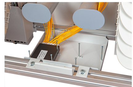
MDO Splitter Box
