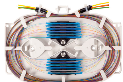
KM 6 (for splicing, up to 24 splices)
